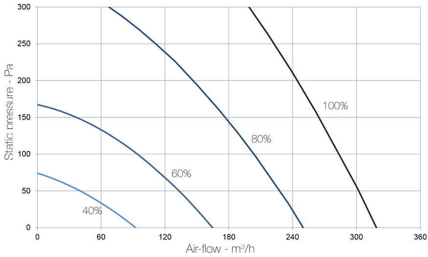
Intake curve according to Reg.1253/2014 (ErP).
